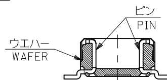
SECT.W-W(LOCK PART)
