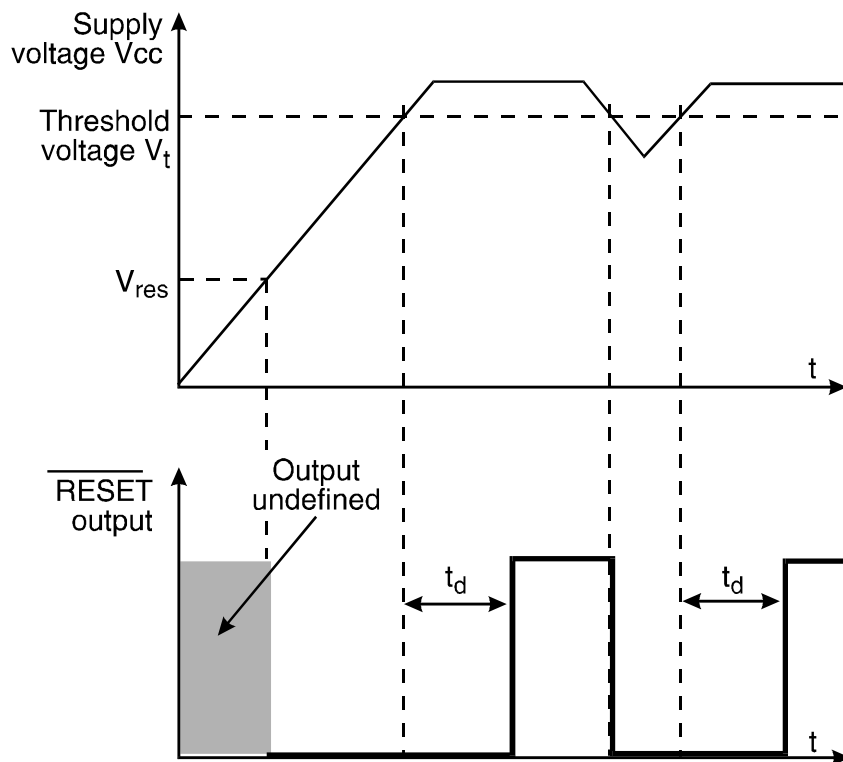
Figure 7. Timing Diagram
