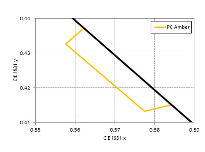
Figure 9. Color bin structure for LUXEON CZ PC Amber for Table 10.
