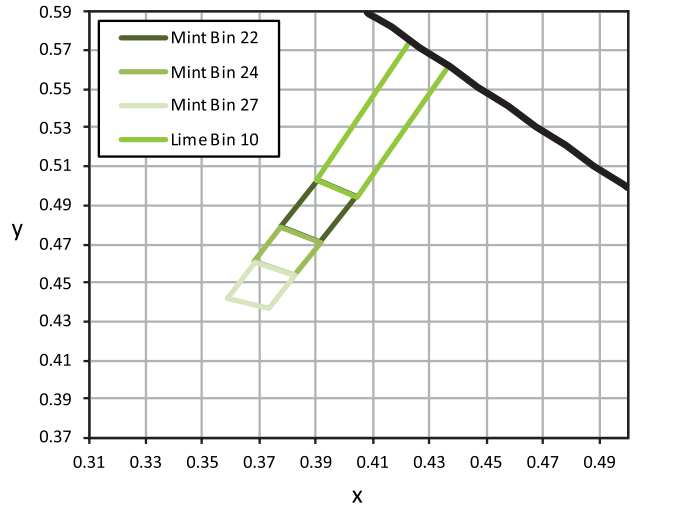
Figure 10. Color bin structure for LUXEON CZ Mint and Lime for Table 10.
