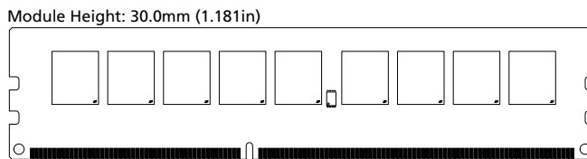
Figure 2: 240-Pin UDIMM (MO-269 R/C D1)
