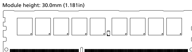
Figure 2: 240-Pin UDIMM (MO-269 R/C D1)
