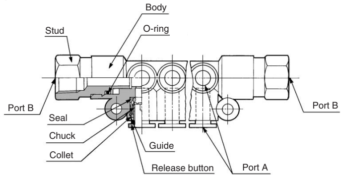
Port A: One-touch fitting Port B: Rc female thread
