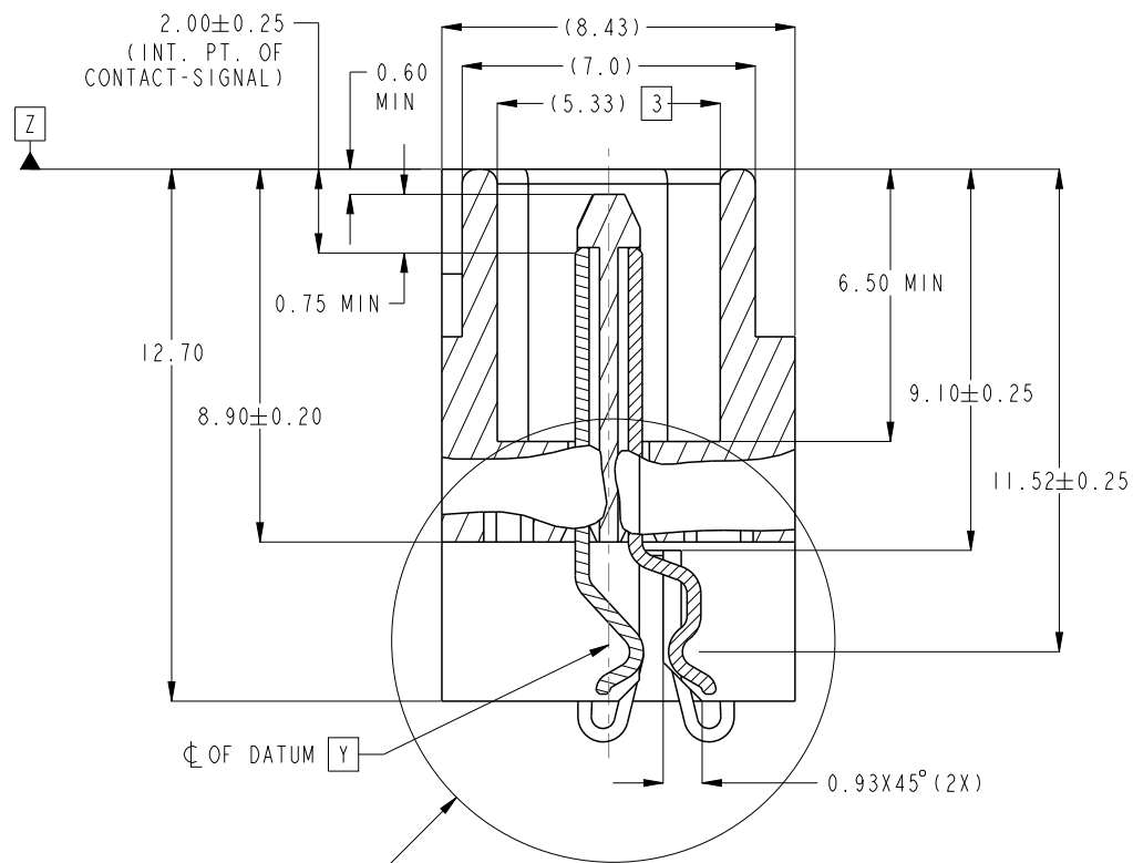
SECTION G-G SCALE 5:1
