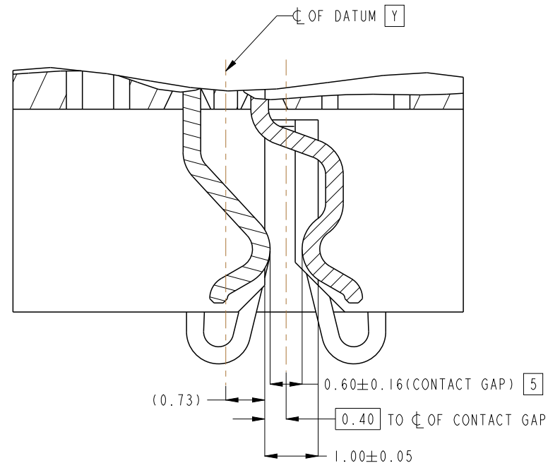
DETAIL D SCALE 10:1
