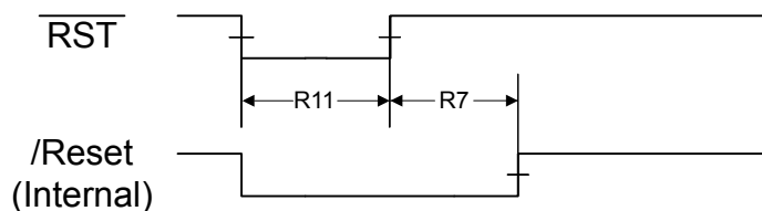
Figure 19-5. External Reset Timing (RST)
