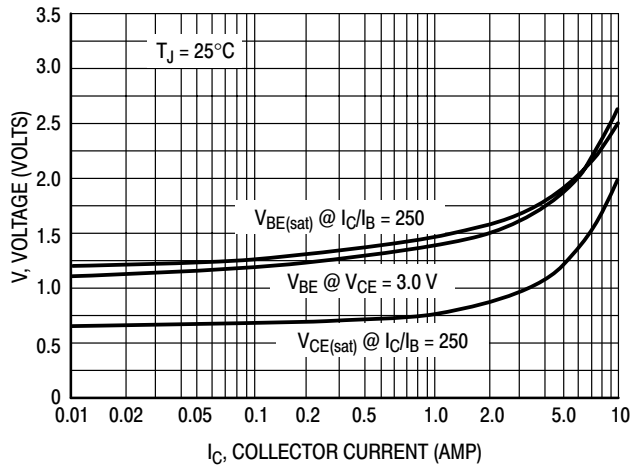
Figure 4. "On" Voltages
