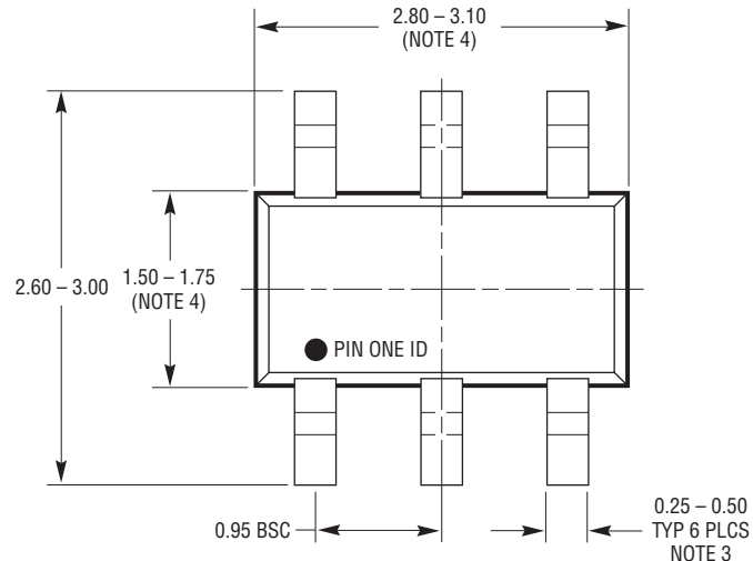
S6 Package 6-Lead Plastic SOT-23 (Reference LTC DWG # 05-08-1634)
