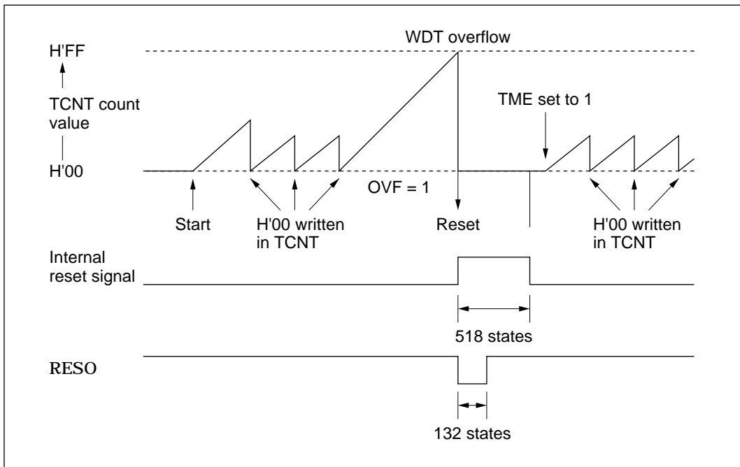
Figure 10-4 Watchdog Timer Operation
