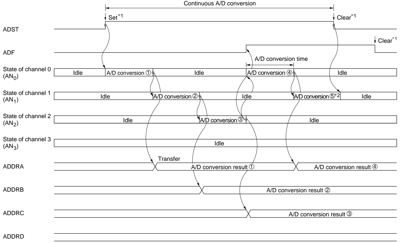
Figure 12-4 Example of A/D Converter Operation (Scan Mode, Channels AN 0 to AN 2 Selected)
