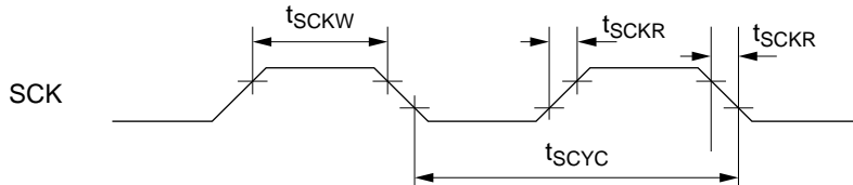
Figure 17-14 SCK Input Clock Timing
