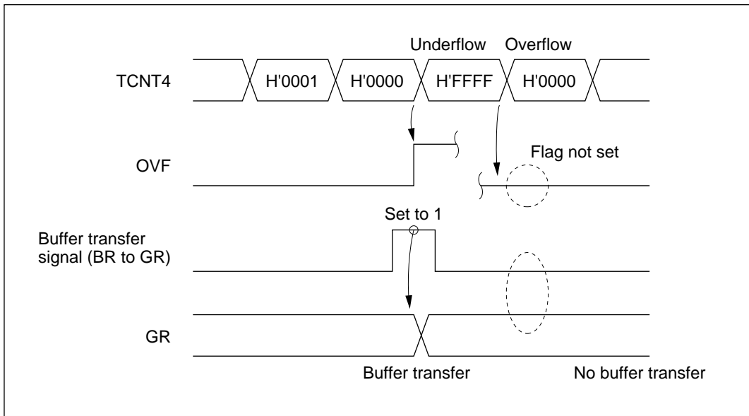
Figure 8-38 Undershoot Timing
