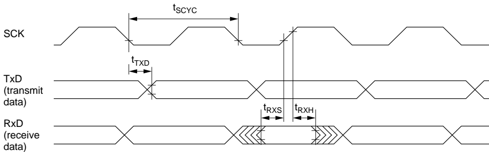
Figure 17-15 SCI Input/Output Timing in Synchronous Mode
