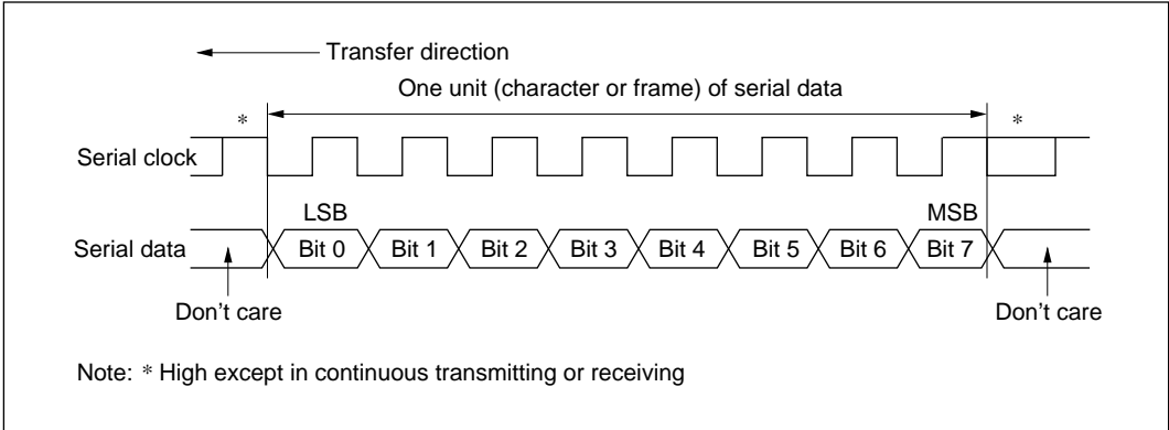
Figure 11-14 Data Format in Synchronous Communication
