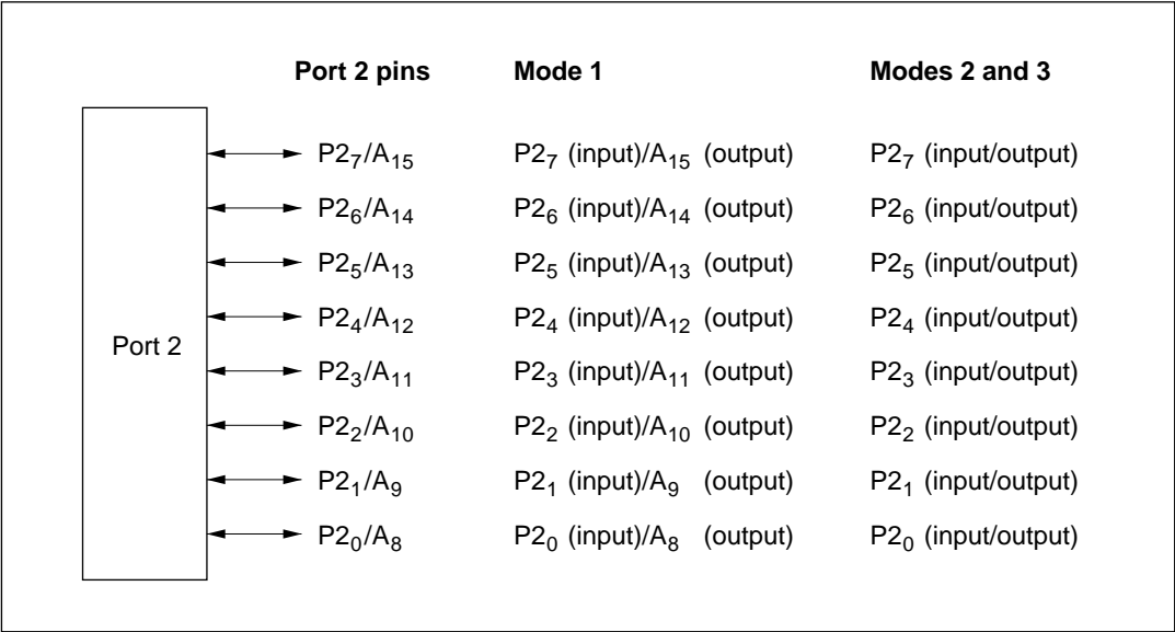
Figure 7-4 Port 2 Pin Configuration
