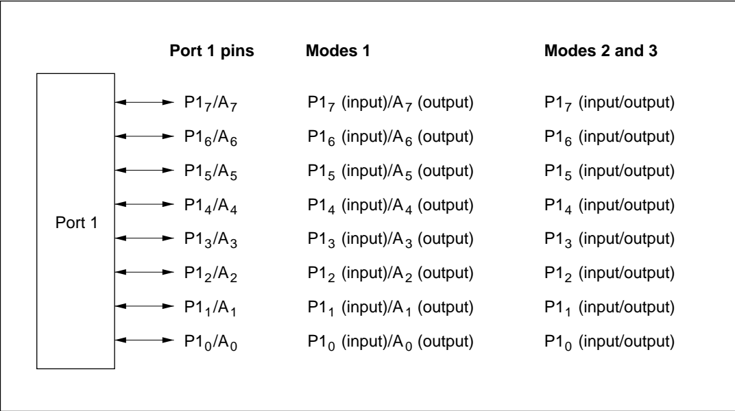
Figure 7-1 Port 1 Pin Configuration
