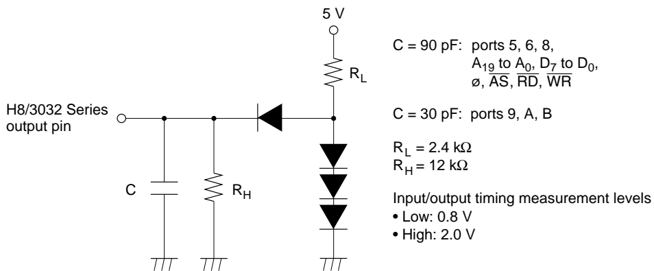
Figure 17-3 Output Load Circuit
