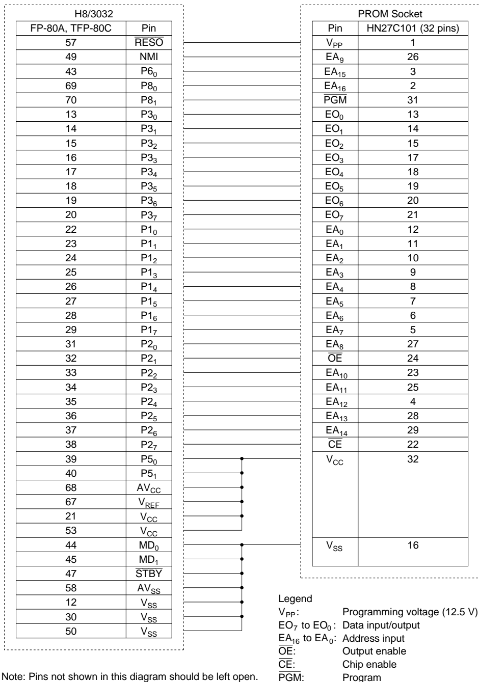
Figure 14-2 Socket Adapter Pin Assignments
