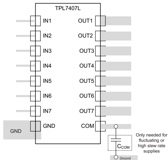
Figure 13. Package Layout
