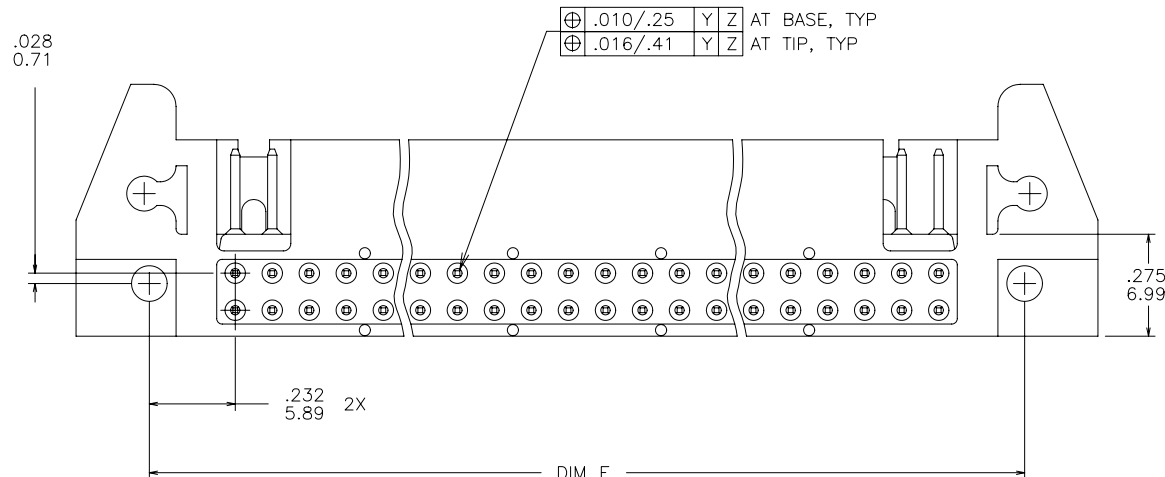
VIEW F-F
