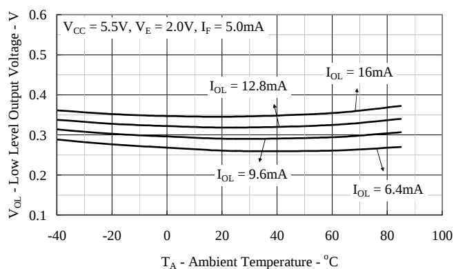
Figure 7: Typical Low Level Output Voltage vs. Ambient Temperature
