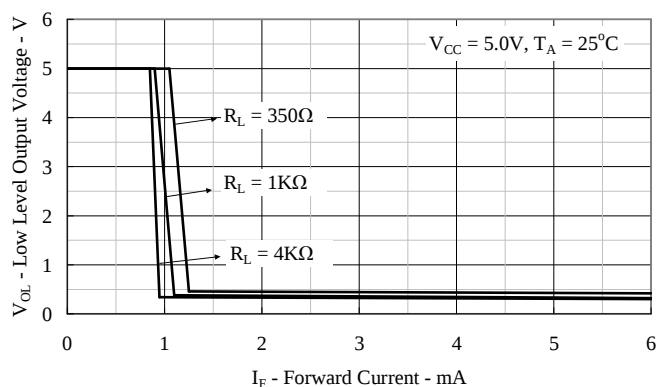
Figure 6: Typical Output Voltage vs. Input Forward Current
