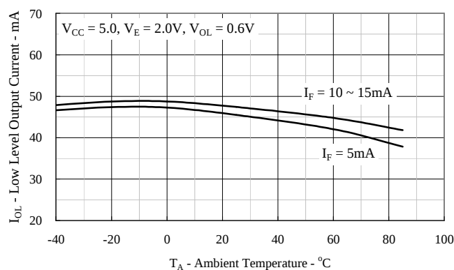
Figure 8: Typical Low Level Output Current vs. Ambient Temperature
