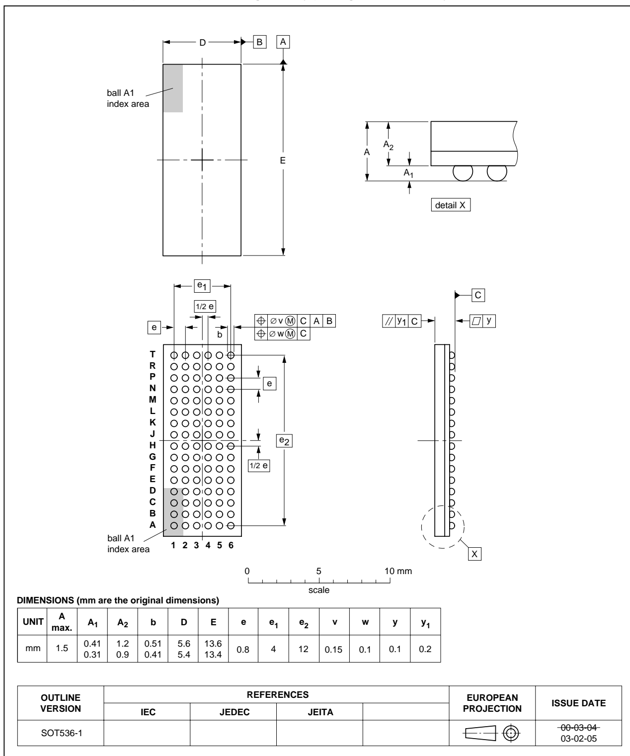
Fig 27. Package outline SOT536-1 (LFBGA96)
