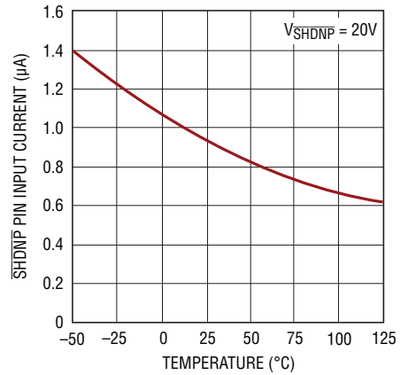
SHDNP Pin Input Current
