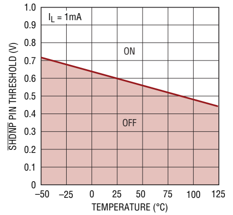
SHDNP Pin Threshold
