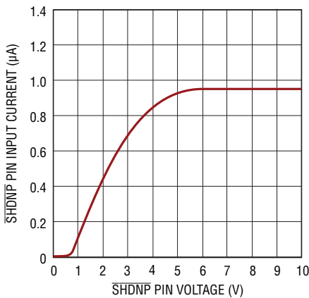
SHDNP Pin Input Current
