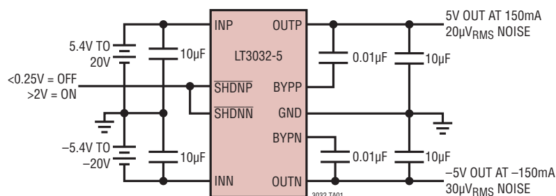
Dual Polarity Low Noise 150mA Power Supply
