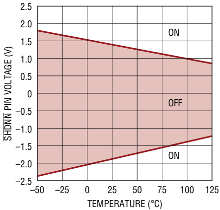
SHDNN Pin Thresholds
