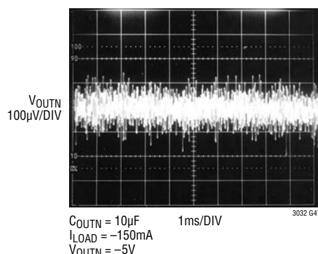
OUTN, 10Hz to 100kHz Output Noise, C_BYPN = 0.01µF
