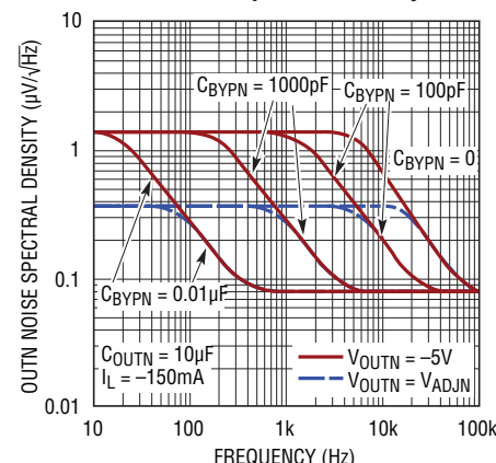
OUTN Noise Spectral Density
