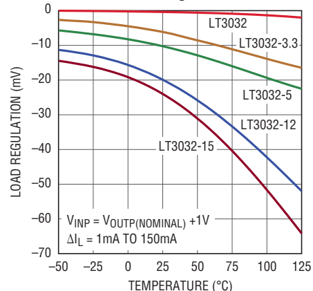
Positive Load Regulation
