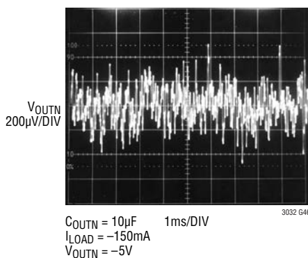
OUTN, 10Hz to 100kHz Output Noise, C_BYPN = 0
