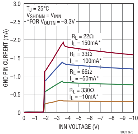
LT3032-3.3 Negative Side GND Pin Current
