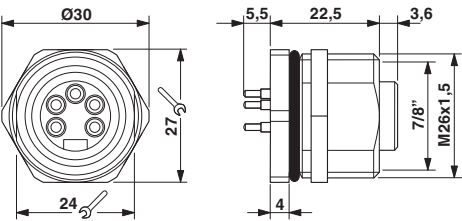
7/8" flush-type socket
