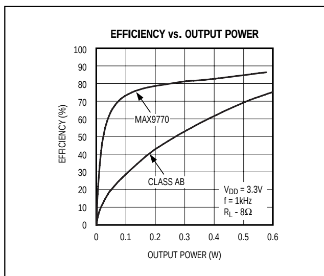
Figure 5. MAX9770 Efficiency vs. Class AB Efficiency
