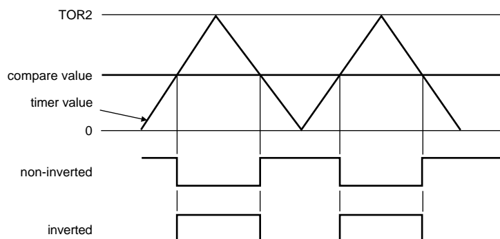
Fig 9. Symmetrical PWM.
