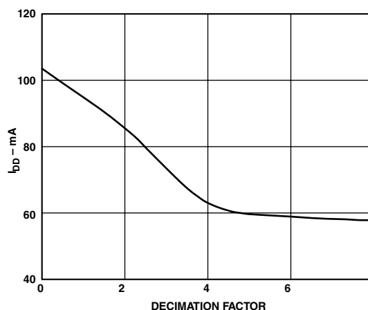
Figure 22. I_{DD} vs. Decimation for a Filter with a Transition Width of 66 kHz as Shown in Figure 1
