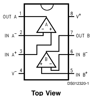
Connection Diagram 8-Pin DIP/SO
