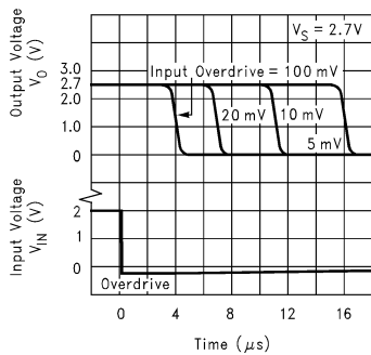
Response Time for Overdrive ( t_{PHL} )
