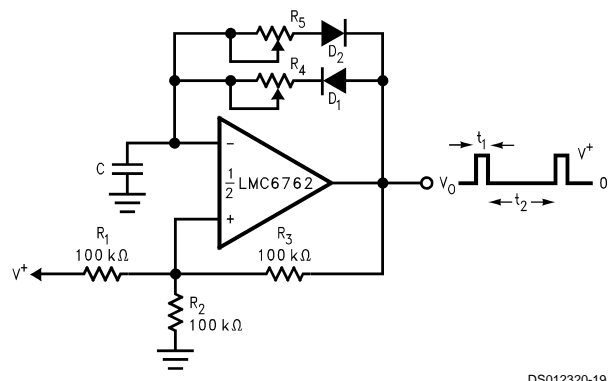
FIGURE 9. Square Wave Generator
