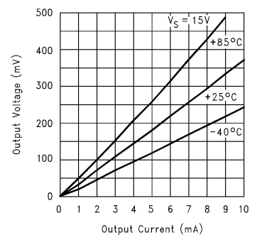
Output Voltage vs Output Current (Sinking)
