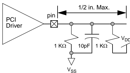
Figure 6-5. PCI Slew Rate Test Circuit
