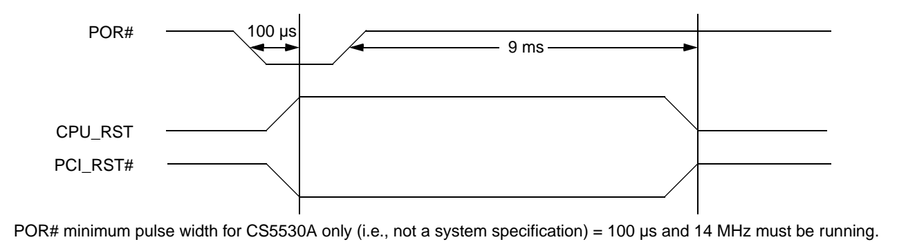
Figure 4-5. CS5530A Reset
