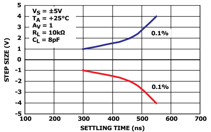
FIGURE 26. STEP SIZE vs SETTLE TIME
