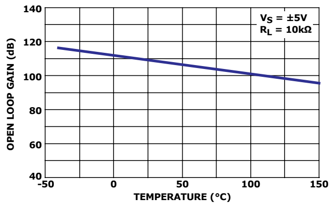
FIGURE 10. OPEN-LOOP GAIN vs TEMPERATURE
