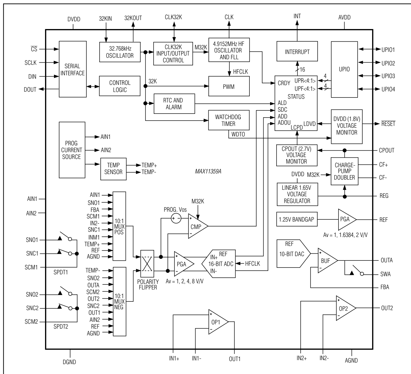
Figure 3. MAX11358B Functional Diagram
