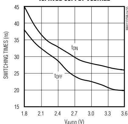
SPDT/SPST SWITCHING TIME vs. AVDD SUPPLY VOLTAGE
