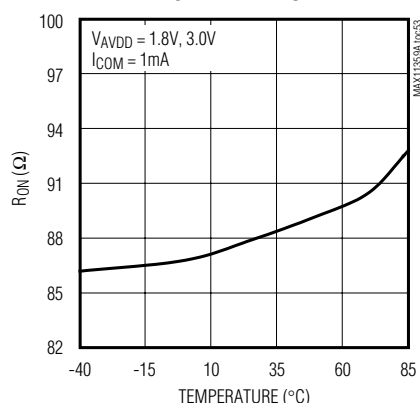
SPST ON-RESISTANCE vs. TEMPERATURE
