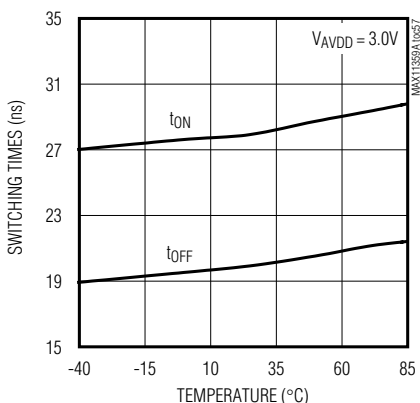
SPDT/SPST SWITCHING TIME vs. TEMPERATURE
