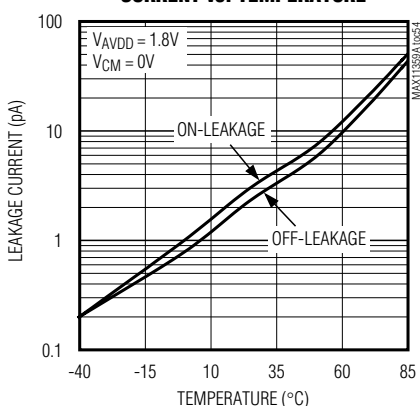
SPDT/SPST ON/OFF-LEAKAGE CURRENT vs. TEMPERATURE
