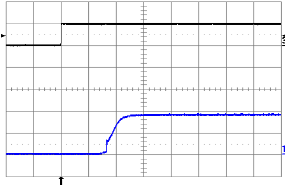
Fig. 1.8V.3: Turn-on transient at full rated load current (resistive) with no output capacitor at V_{in} = 48\text{ V} , triggered via ON/OFF pin. Top trace: ON/OFF signal (5 V/div.). Bottom trace: output voltage (1 V/div.). Time scale: 1 ms/div.
