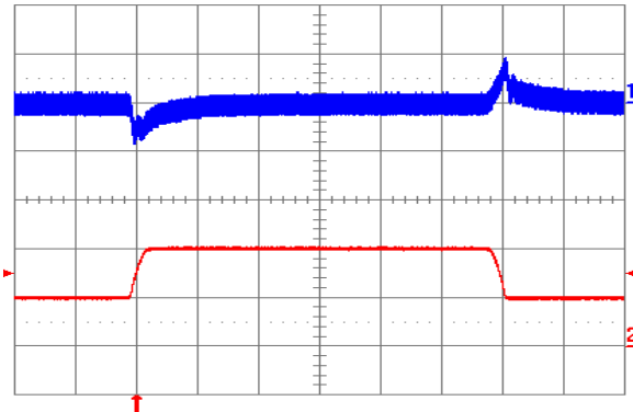
Fig. 2.5V.5: Output voltage response to load current step-change (5 A – 10 A – 5 A) at V_{in} = 48 V. Top trace: output voltage (100 mV/div.). Bottom trace: load current (5 A/div.). Current slew rate: 0.1 A/ \mu s. C_o = 1 \mu F ceramic. Time scale: 0.2 ms/div.
