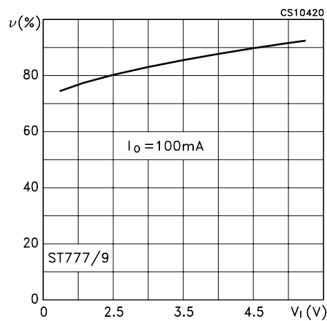
Figure 5 : Efficiency vs Output Current
