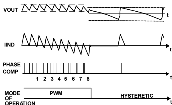
FIGURE 35. CCM—HYSTERETIC TRANSITION
