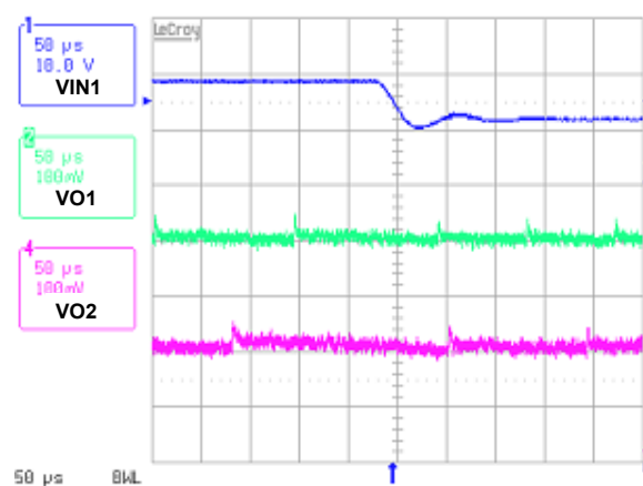
FIGURE 14. INPUT STEP-DOWN TRANSIENT AT HYS MODE
