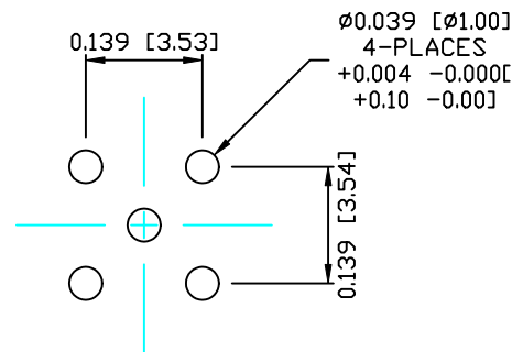
PLC LAYOUT
