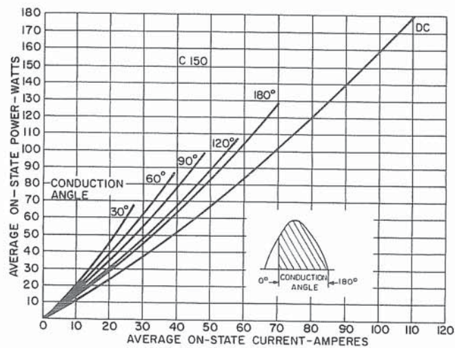
2. MAXIMUM ON-STATE POWER DISSIPATION FOR SINUSOIDAL CURRENT WAVEFORM
