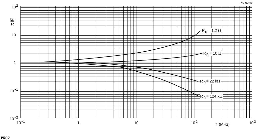
Fig.36 Impedance as a function of applied frequency.
