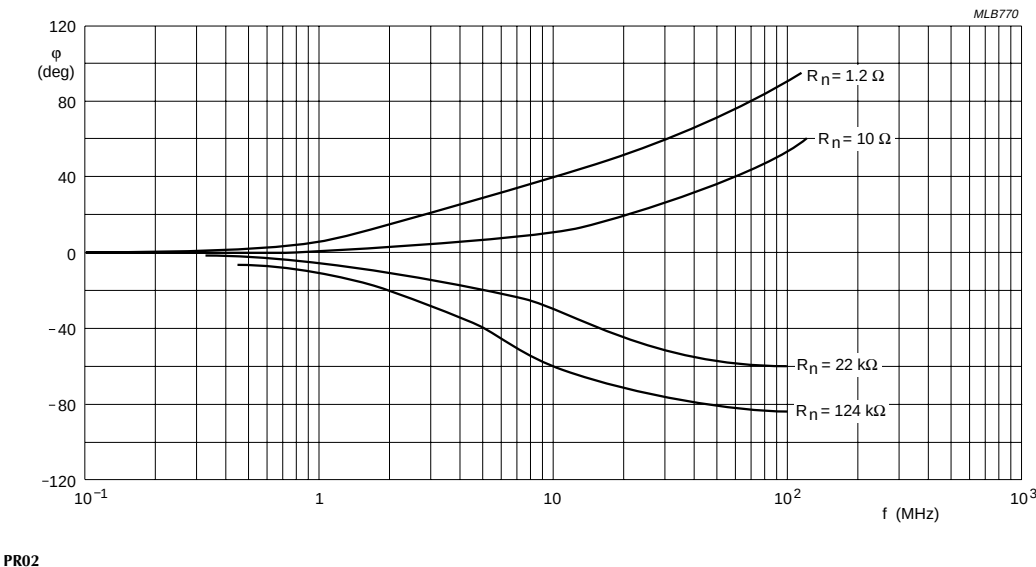
Fig.37 Phase angle as a function of applied frequency.
