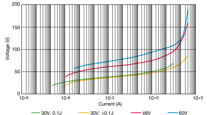
VI Curves - 30V, 48V, and 60V Products
