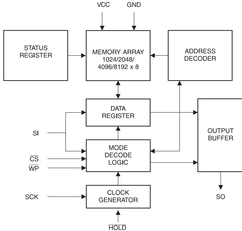
Figure 1. Block Diagram
