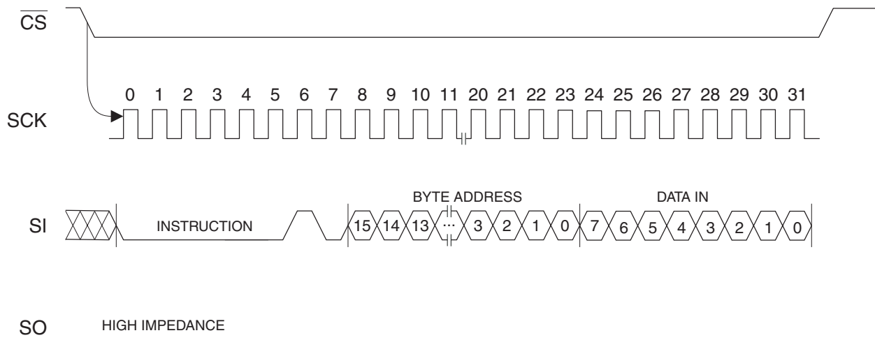
Figure 9. WRITE Timing
