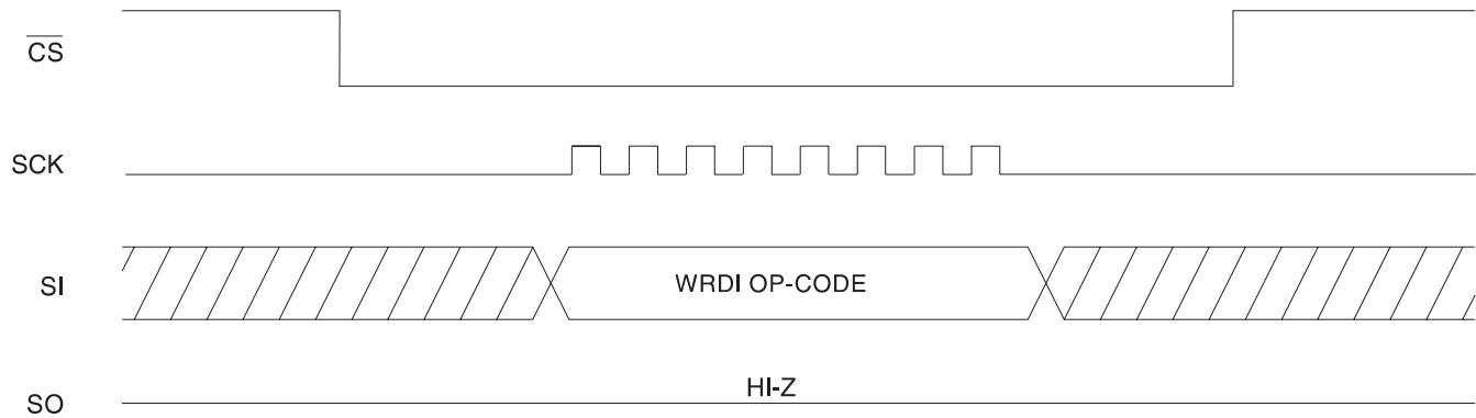
Figure 5. WRDI Timing
