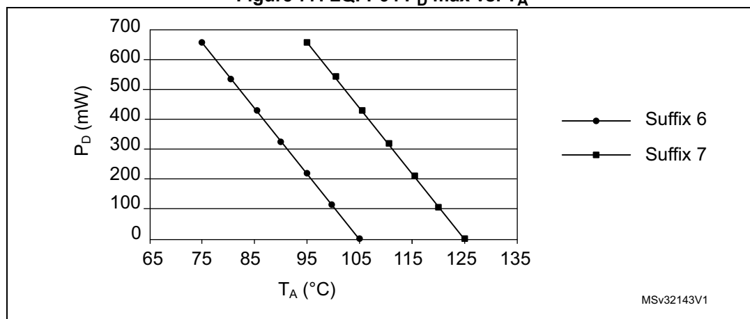
Figure 77. LQFP64 P_D max vs. T_A
