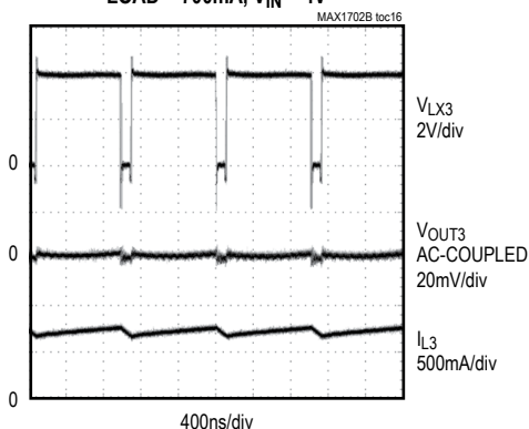
REG3 MEDIUM-LOAD SWITCHING WAVEFORM
