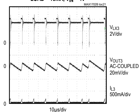
REG3 LIGHT-LOAD SWITCHING WAVEFORM
