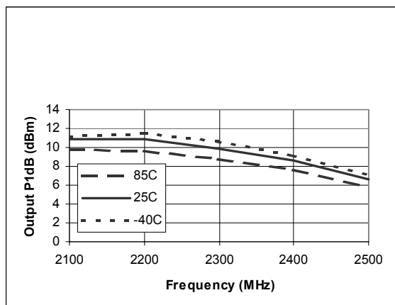
Figure 10. Output P1dB versus Frequency + Temperature
