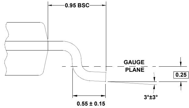
DETAIL "X"
