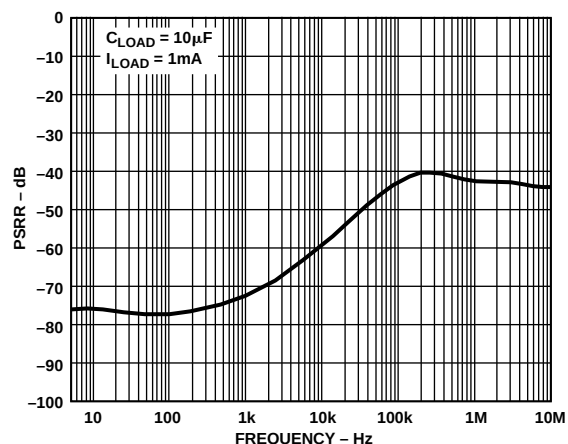
Figure 12. Ripple Rejection*
