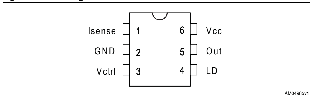
Figure 2. Pin configuration
