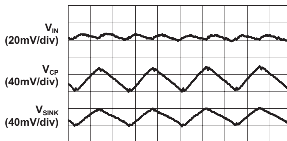
Load Characteristics ( V_{IN} = 2.9V ; 2X Mode; 14mA/ch Load)
