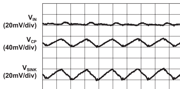
Load Characteristics ( V_{IN} = 3.5V ; 1.5X Mode; 14mA/ch Load)
