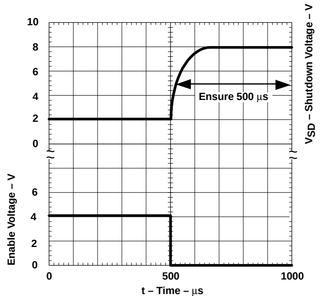
Figure 7. SD Timings
