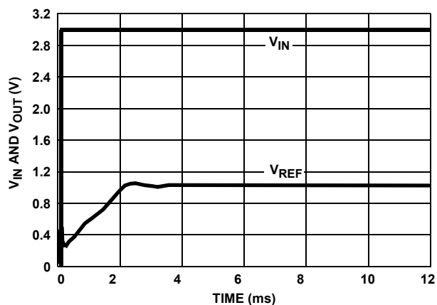
FIGURE 13. TURN-ON TIME ( +25^\circ C )
