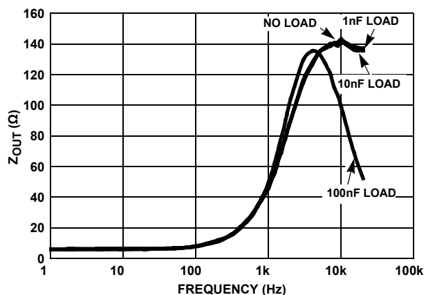
FIGURE 27. Z_{OUT} vs FREQUENCY
