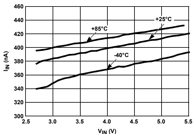
FIGURE 30. I_{IN} vs V_{IN} OVER-TEMPERATURE
