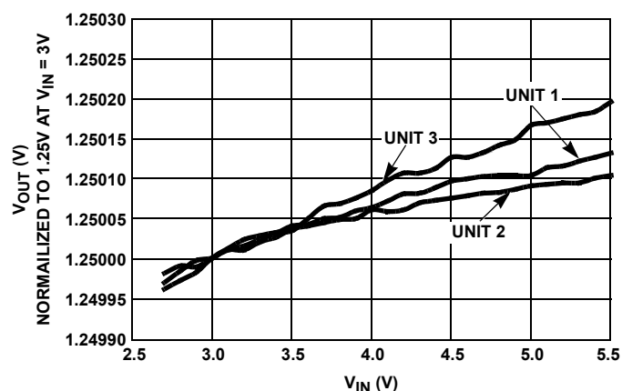
FIGURE 32. LINE REGULATION, 3 UNITS
