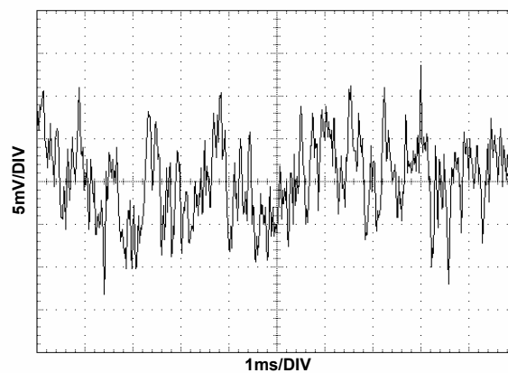
FIGURE 56. V_{OUT} NOISE
