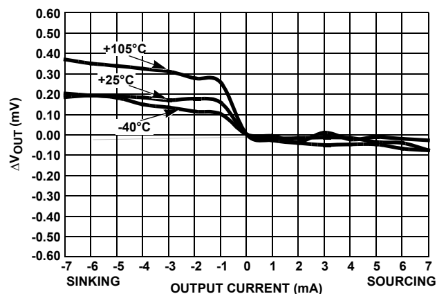
FIGURE 107. LOAD REGULATION
