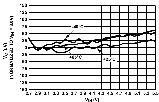
FIGURE 5. LINE REGULATION OVER-TEMPERATURE
