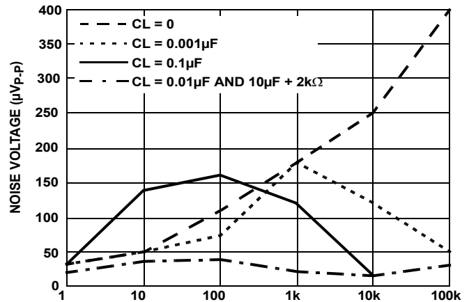
FIGURE 118. NOISE REDUCTION
