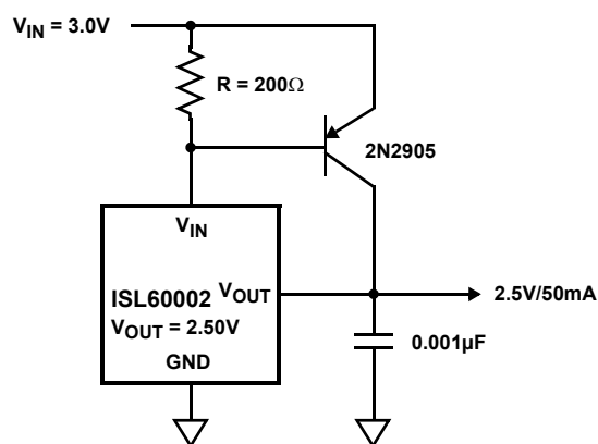
FIGURE 121. PRECISION 2.5V 50mA REFERENCE
