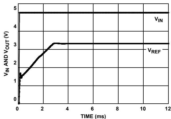
FIGURE 113. TURN-ON TIME (+25°C)
