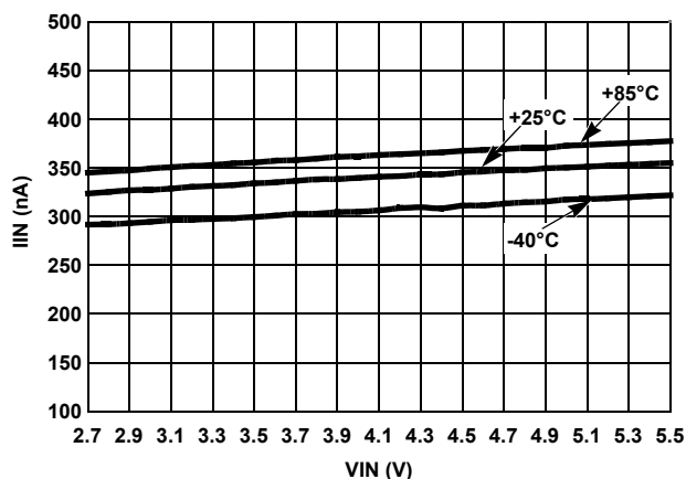
FIGURE 3. I_{IN} vs V_{IN} OVER-TEMPERATURE
