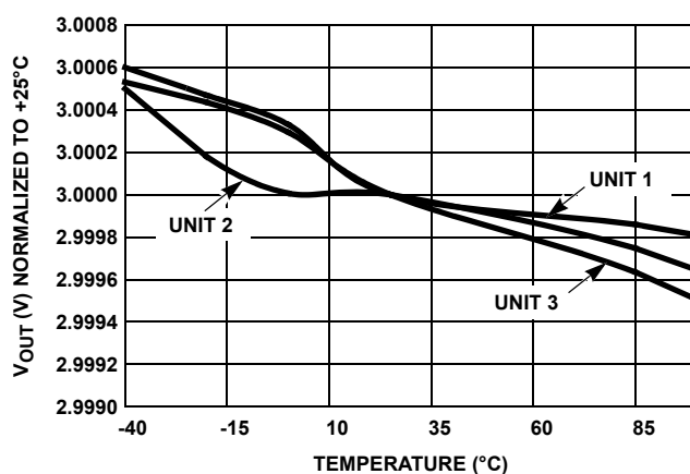
FIGURE 86. V_{OUT} vs TEMPERATURE NORMALIZED TO +25^\circ C
