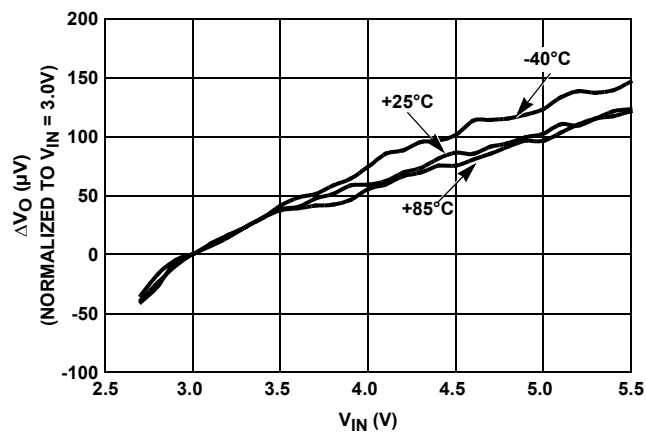
FIGURE 74. LINE REGULATION OVER-TEMPERATURE
