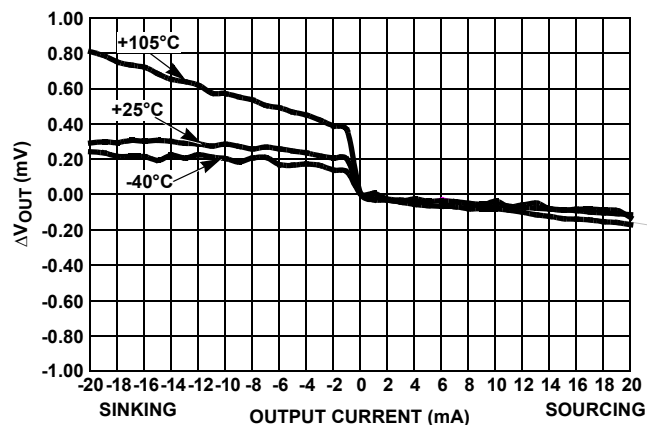
FIGURE 108. LOAD REGULATION OVER-TEMPERATURE
