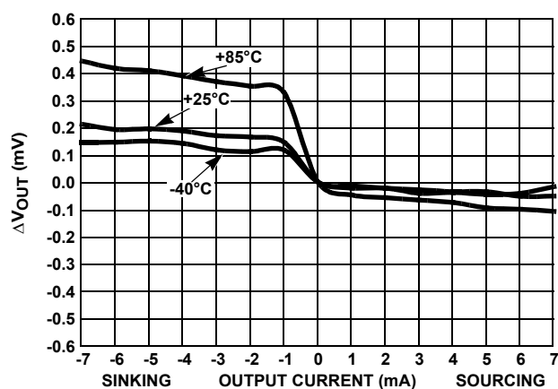
FIGURE 23. LOAD REGULATION OVER-TEMPERATURE
