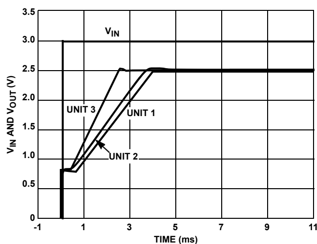
FIGURE 120. TURN-ON TIME
