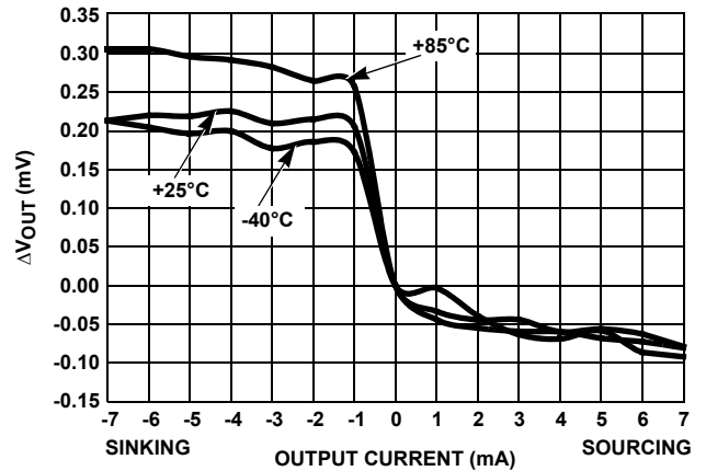
FIGURE 92. LOAD REGULATION OVER-TEMPERATURE
