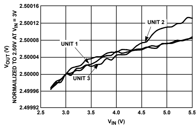
FIGURE 73. LINE REGULATION, 3 UNITS
