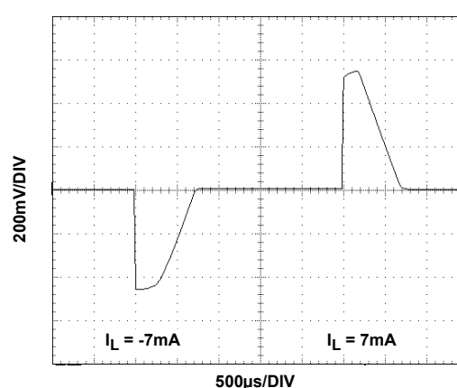
FIGURE 25. LOAD TRANSIENT RESPONSE
