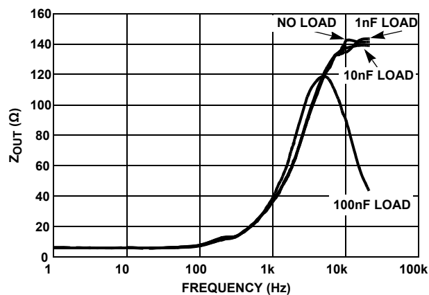
FIGURE 98. Z_{OUT} vs FREQUENCY
