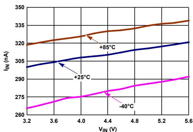
FIGURE 85. I_{IN} vs V_{IN} OVER-TEMPERATURE
