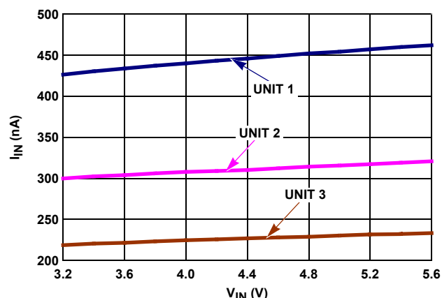
FIGURE 84. I_{IN} vs V_{IN} , 3 UNITS
