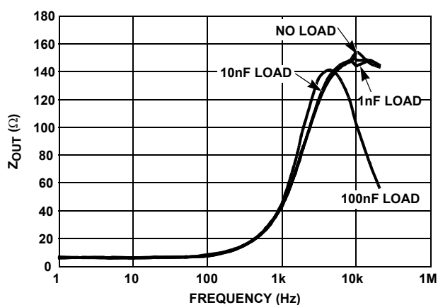
FIGURE 41. Z_{OUT} vs FREQUENCY
