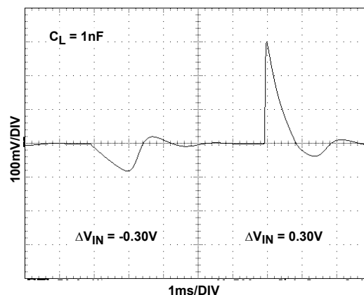
FIGURE 35. LINE TRANSIENT RESPONSE, WITH CAPACITIVE LOAD
