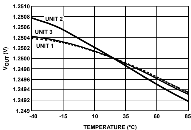
FIGURE 31. V_{OUT} vs TEMPERATURE NORMALIZED TO +25^\circ C
