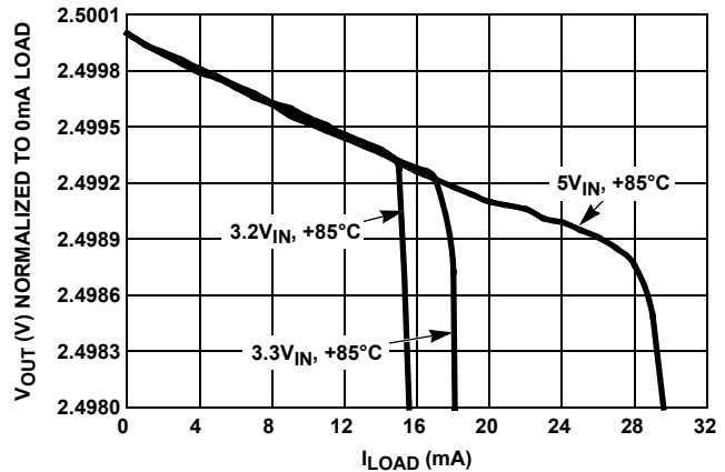
FIGURE 116. DIFFERENT V_{IN} AT HIGH TEMPERATURE
