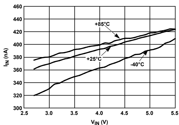
FIGURE 71. I_{IN} vs V_{IN} OVER-TEMPERATURE
