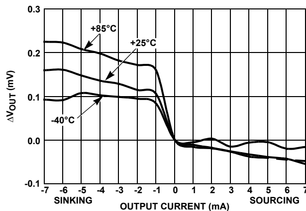
FIGURE 37. LOAD REGULATION
