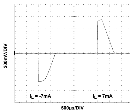
FIGURE 39. LOAD TRANSIENT RESPONSE
