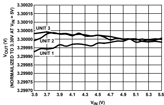
FIGURE 102. LINE REGULATION, 3 UNITS
