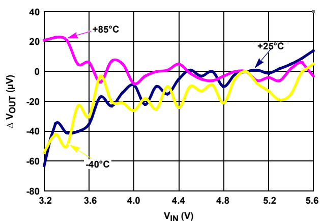
FIGURE 88. LINE REGULATION OVER-TEMPERATURE
