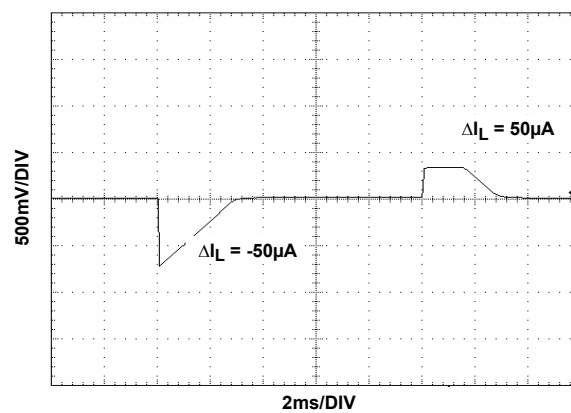
FIGURE 66. LOAD TRANSIENT RESPONSE
