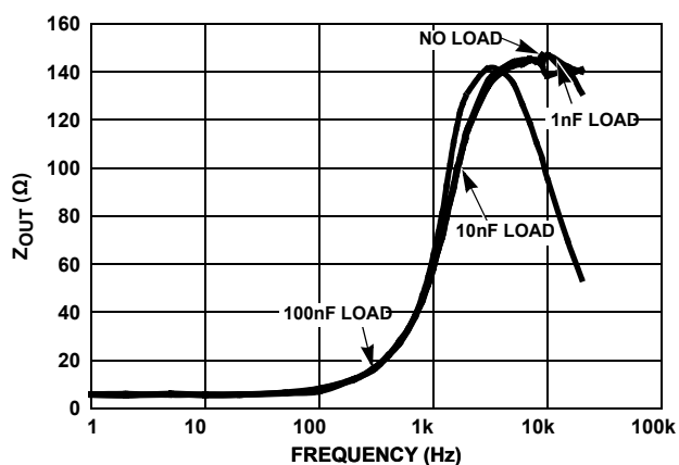
FIGURE 14. Z_{OUT} vs FREQUENCY
