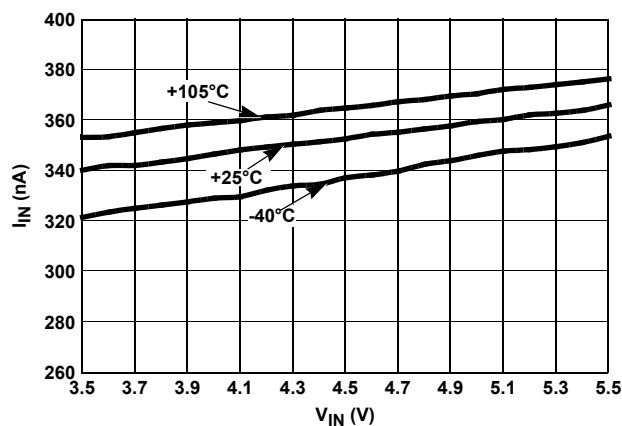
FIGURE 100. I_{IN} vs V_{IN} OVER-TEMPERATURE
