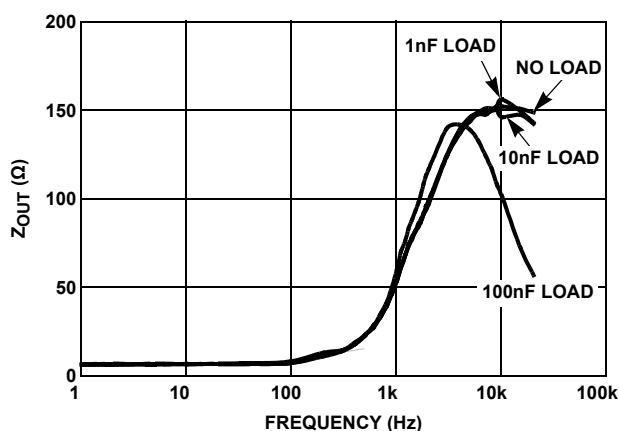
FIGURE 82. Z_{OUT} vs FREQUENCY
