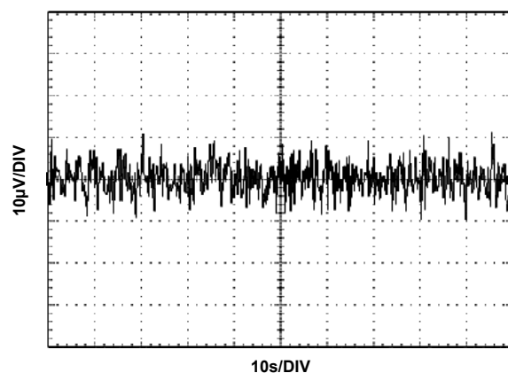
FIGURE 83. V_{OUT} NOISE
