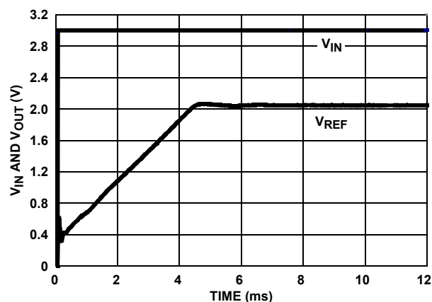
FIGURE 68. TURN-ON TIME ( +25^\circ C )
