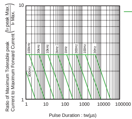
Fig.4 Ratio of Maximum Tolerable Peak Current - Pulse Duration ( I )
