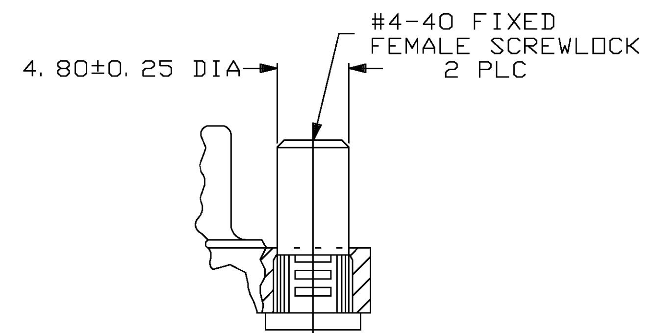
Detail A
