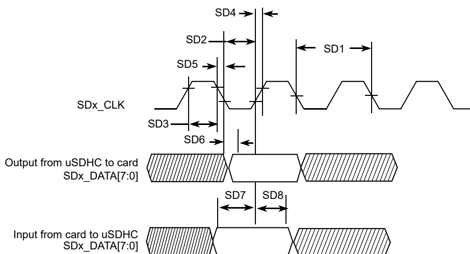
Figure 36. SD/eMMC4.3 timing
