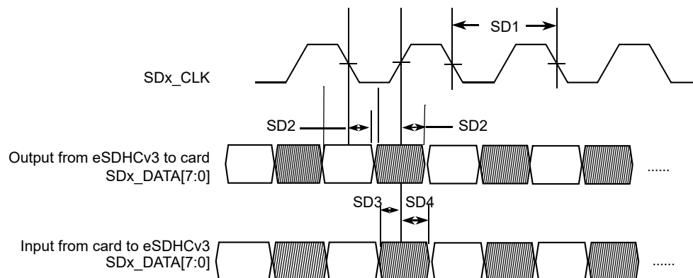
Figure 37. eMMC4.4/4.41 timing
