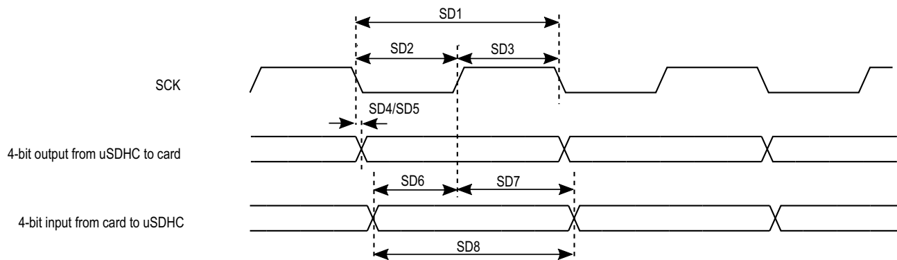
Figure 38. SDR50/SDR104 timing
