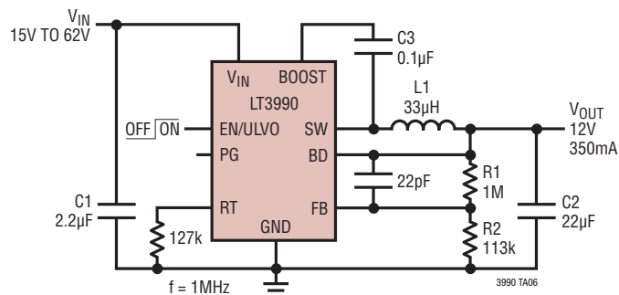
12V Step-Down Converter
