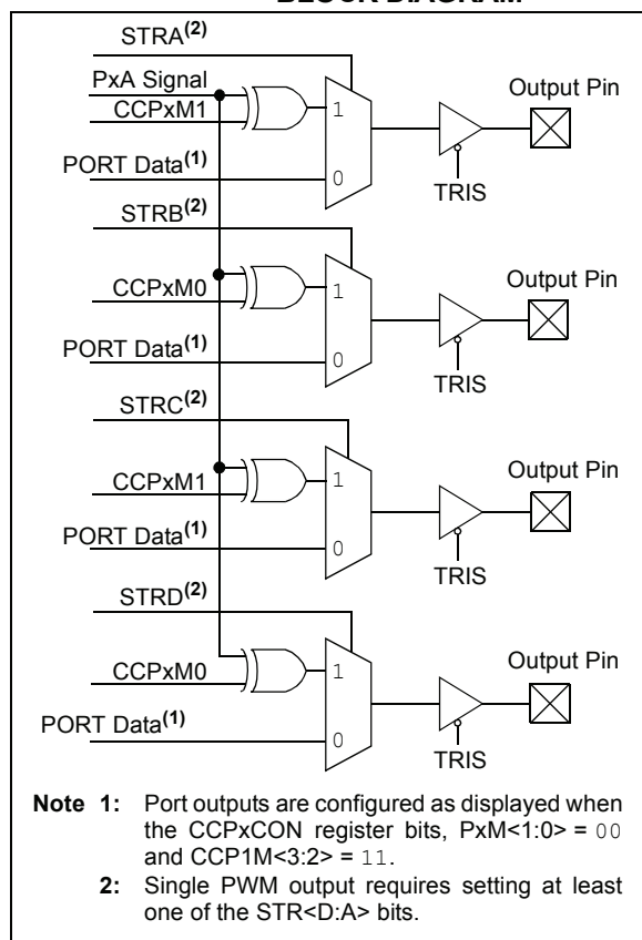
FIGURE 19-16: SIMPLIFIED STEERING BLOCK DIAGRAM
