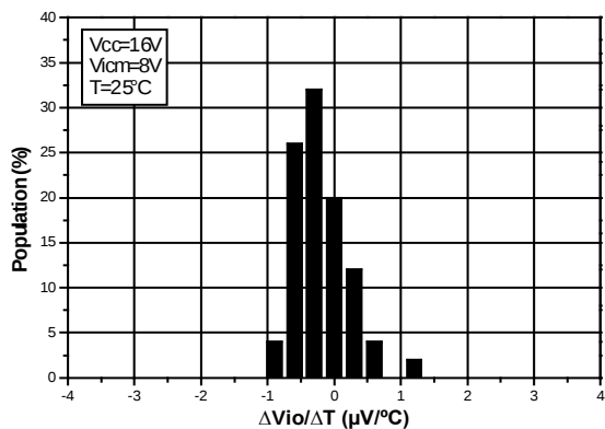
Figure 6: Input offset voltage drift population
