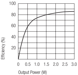
Channel Vo3 (nominal 72V)
