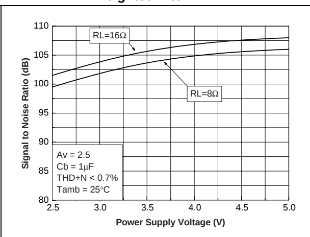
Figure 68. SNR vs. power supply voltage with A-weighted filter
