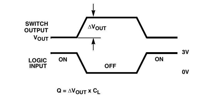
FIGURE 1. SWITCHING TIMES
