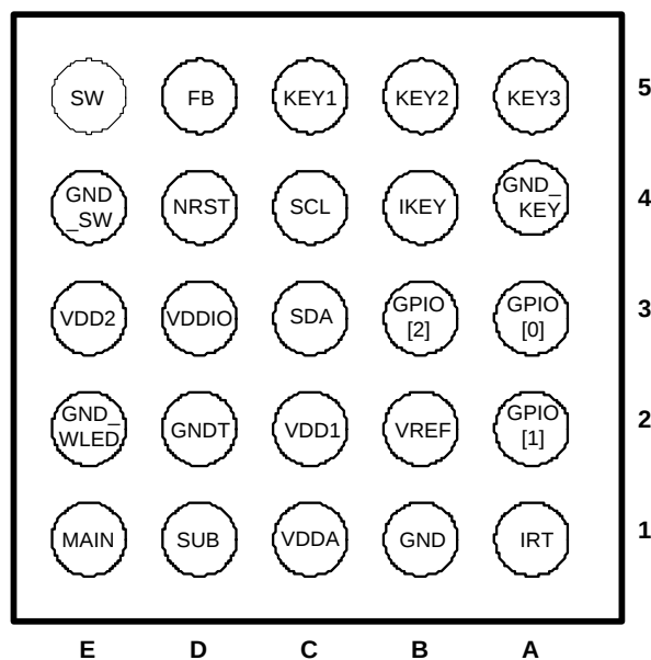
Figure 2. Bottom View
