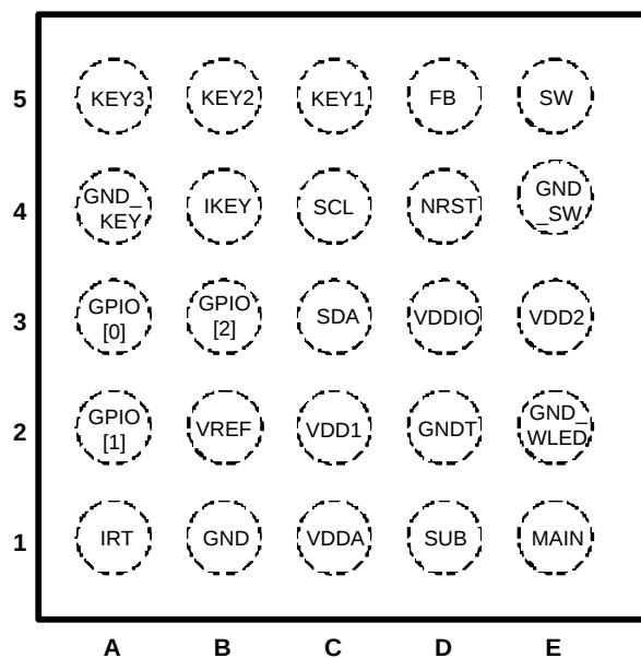
Figure 1. Top View
